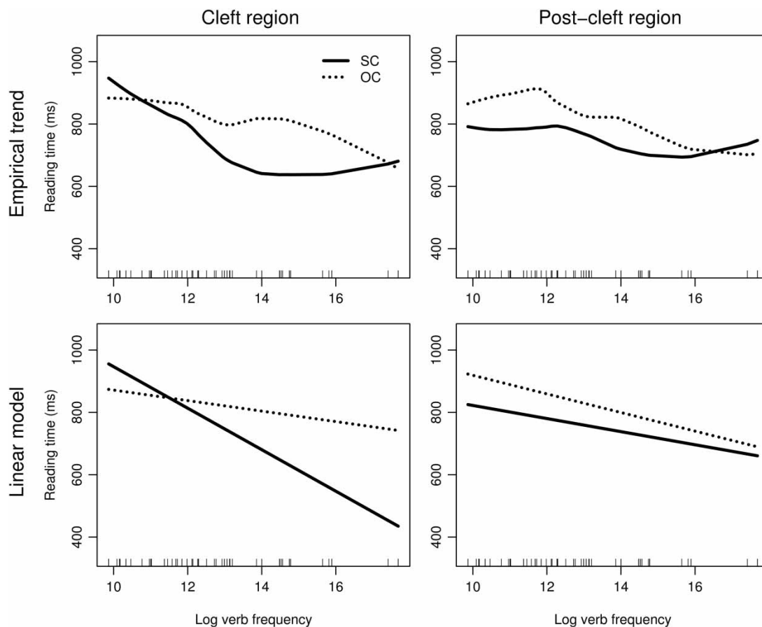
Figure 3. The model predictions (two lower panels) and the data (two top panels) for the two critical regions: cleft (the left panels) and postcleft (the right panels).
