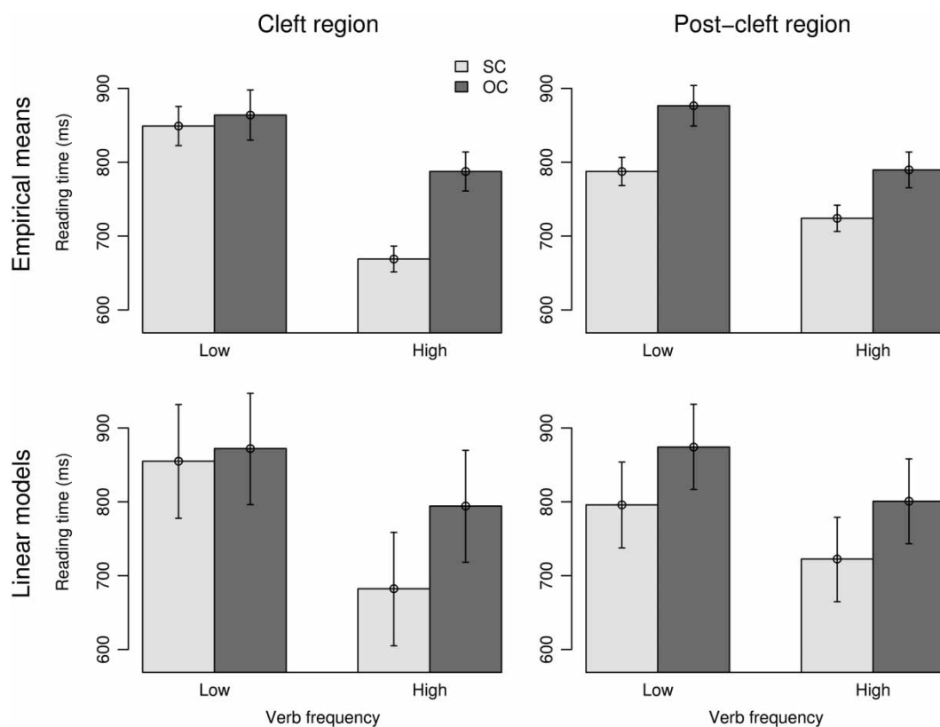
Figure 2. Empirical per-condition means (upper plots, error bars represent two standard errors of the mean) and fitted model predictions for the two linear regression models (lower plots, error bars represent two standard deviations).
