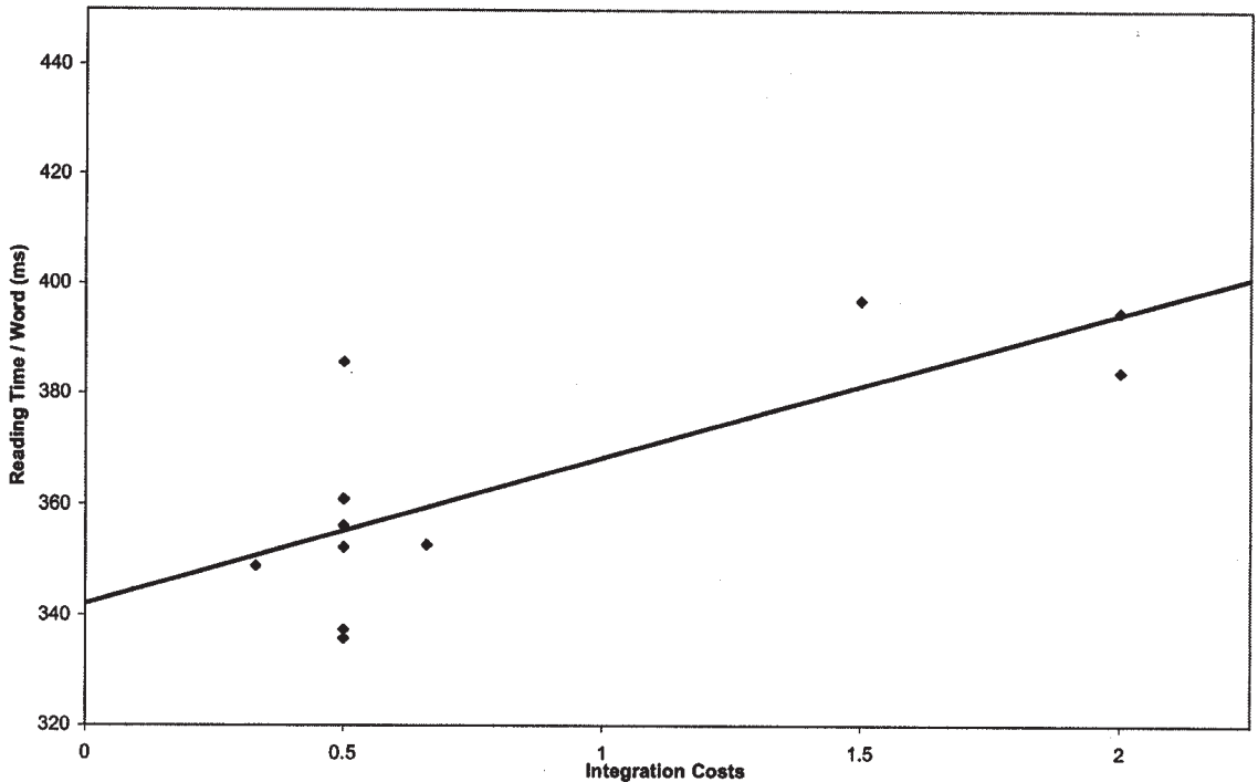
Fig. 1. Locality as a predictor of reading times in Experiment 1 by regions.
