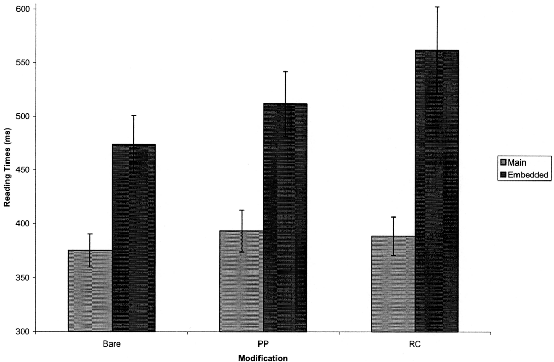
Fig. 3. Average reading times on the verbs in Experiment 2 by condition.
