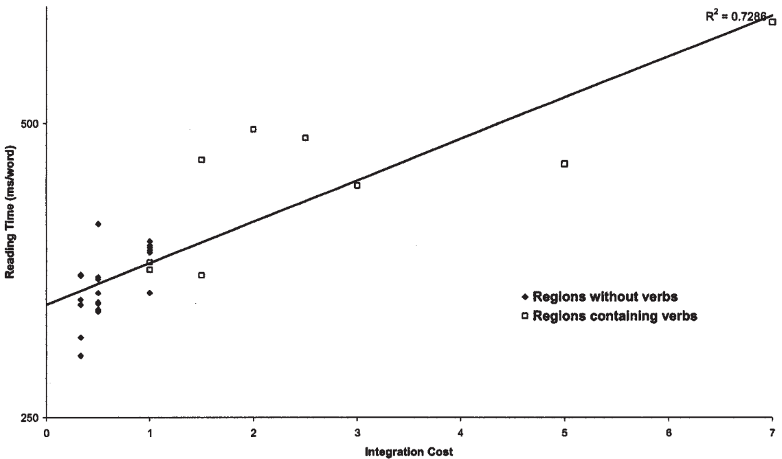
Fig. 6. Integration cost as a linear predictor of reading times per region in Experiment 2.
