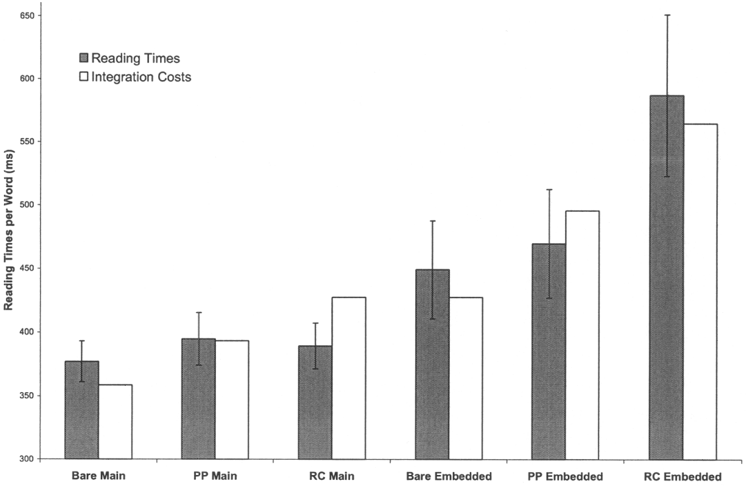
Fig. 4. Reading times and predicted locality costs at the first verb for each condition in Experiment 2 ( r^2 = .889 ).
